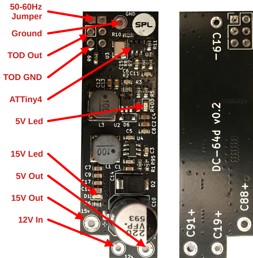
Figure 1: DC-64d Front & Back
