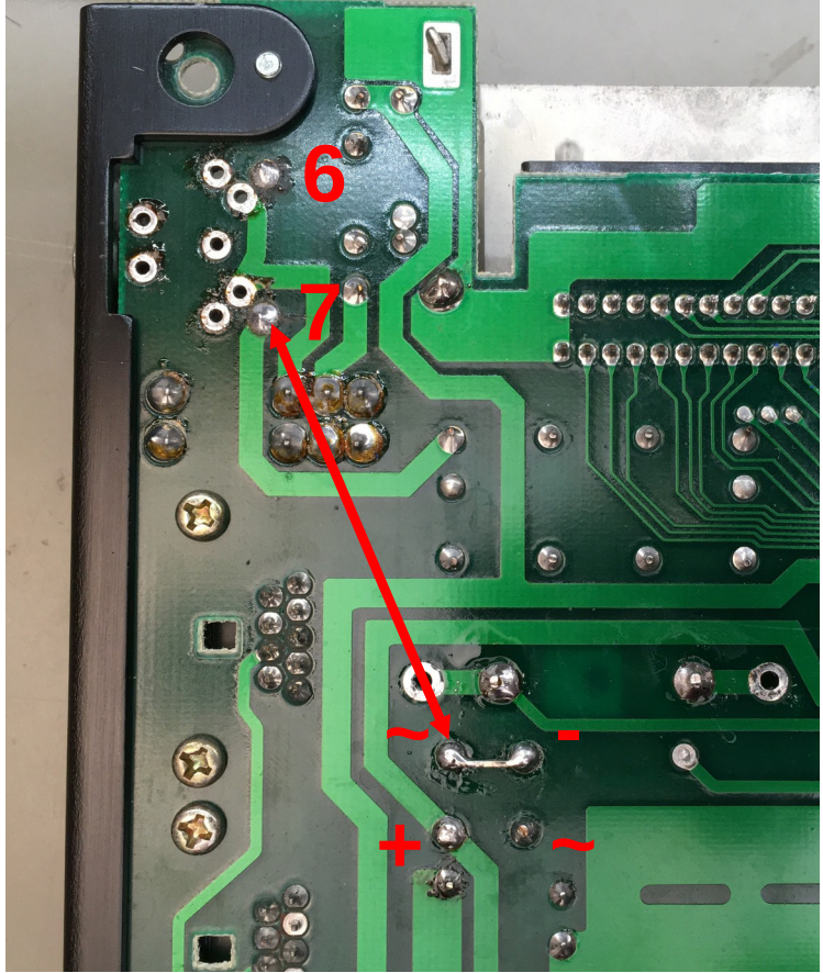
Figure 8: CR4 Rectifier Bypass Example
