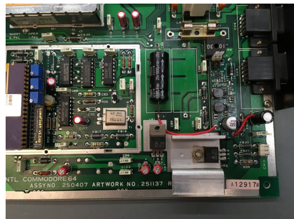
Figure 3: Assy 250407 Installation
