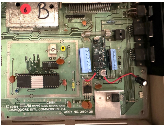
Figure 2: Assy 251425 Installation
